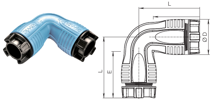
Elbow 90° No. 6420HFA
