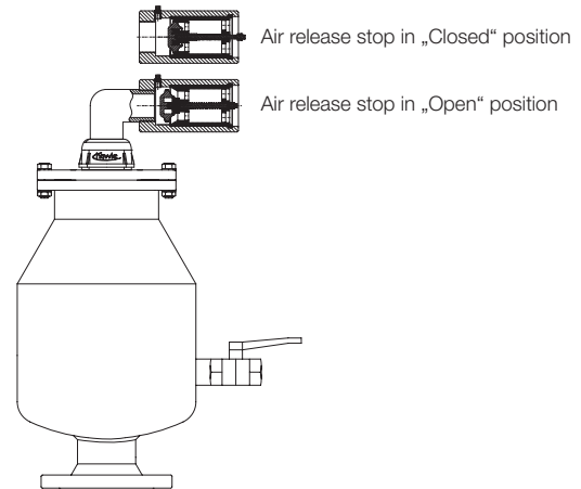
Wastewater automatic air valve with air release stop
