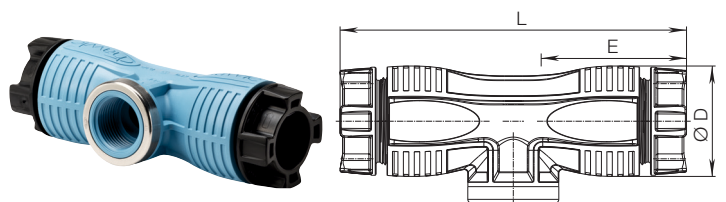
T-piece with threaded outlet No. 6520HFA
