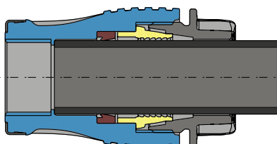
Open clamping nut
