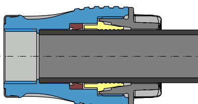
Clamping nut fully tightened
